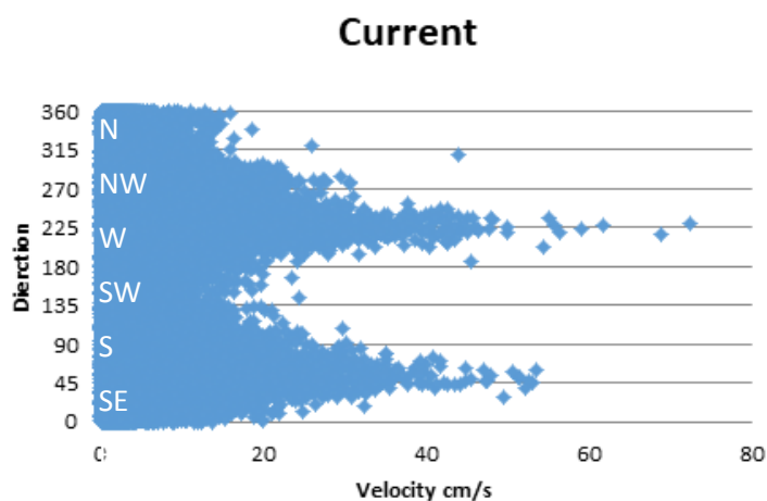
Figure 11: Current velocity and direction measured by an oceanographic instrument at 16 m depth below the farm-site in Byxelkrok, from 2017-11-08 to 2018-08-29. The instrument showed that at some points the current velocities were very high considering incubation depth, up to 1.4 knots. The dominating current direction was NE to SW and opposite, same direction in which the nets were anchored. However, it seemed that the current quite often could come from other directions as well. This caused a lot of extra strain to the construction.
