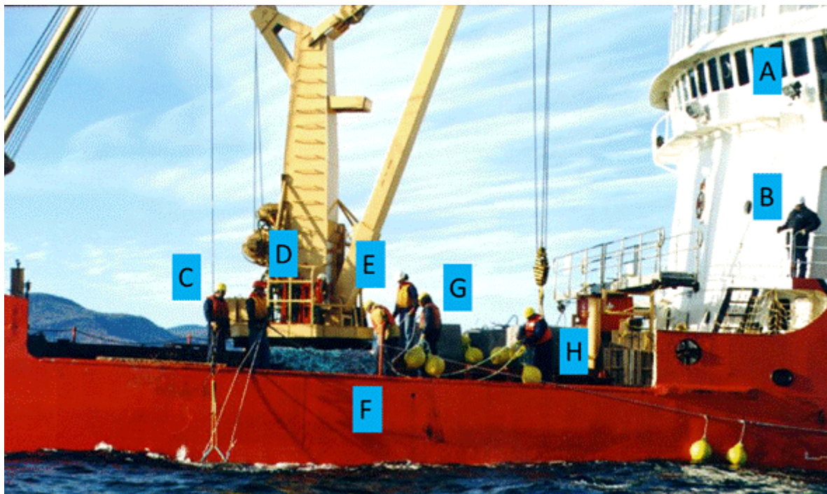
Figure 48 Deployment of the concrete anchors in a longline series from a big ship able to move 3 tons anchor
