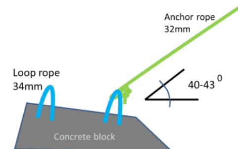
Figure 21 Anchor rope
