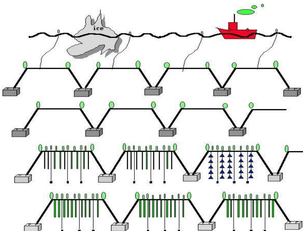
Figure 29 Example - Organisation of a shellfish culture site for submerged longlines (J.Bonardelli)
