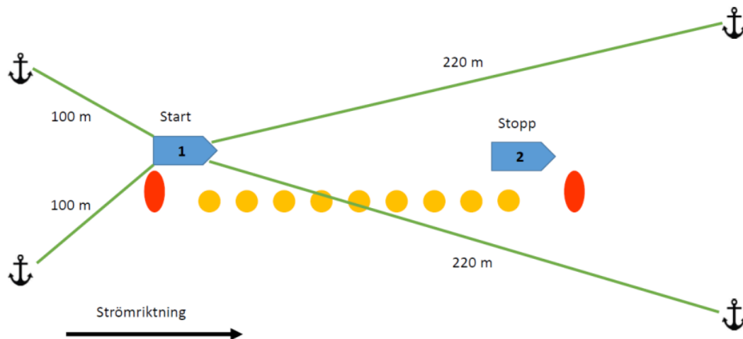
Figure 2. Positioning of the boat at anchor-drilling with help of bruce-anchors, line-pullers and the “pearl-string”.
