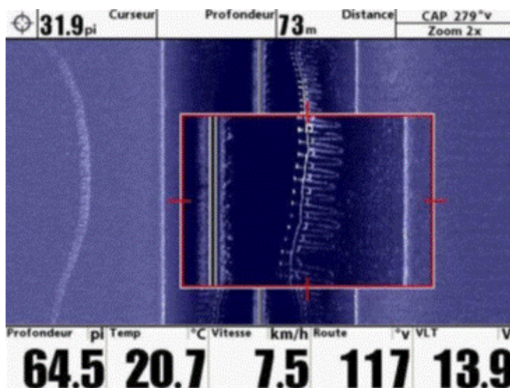
Figure 62 Top image of side-scan sonar of mussel socks on line. This image shows the individual mussel socks as the boat is driving above the submerged longline at 10m below surface. It is possible to see the long and short loops of the continuous mussel ropes ha
