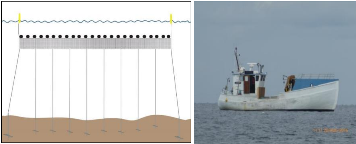
Figure 1. Left: Concept of the Shelltech Offshore farm. Right: The work vessel used
