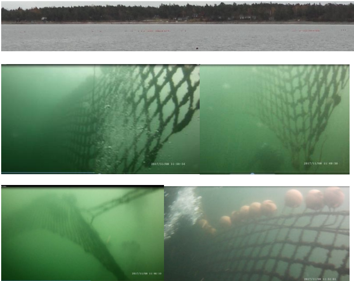
Figure 12: Pictures from the farm site at inspection 2017-11-08. Top: Net 1 and 3 were not visible from the surface, with the exception of 3-5 floats at the site of the broken shack of net 1. Net 2 was still visible as floats coming up between the anchors, due to the stretching of the net. Middle: Note the considerable stretch of the net, partly because of the lack of a direct connection between the attachment of the anchor line and the upper frame of the net. Bottom: Net 3 was fully submerged from 3-6 m depth.
