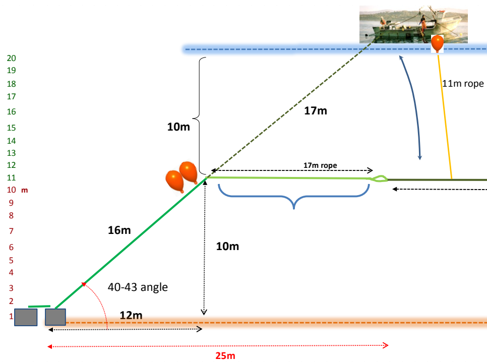
Figure 31 Angle of longline
