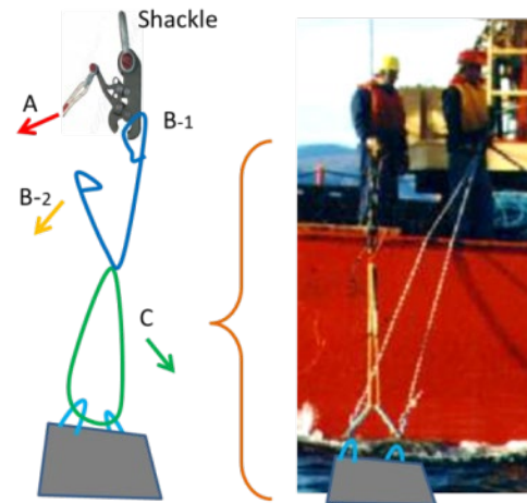
Figure 47 Anchoring
